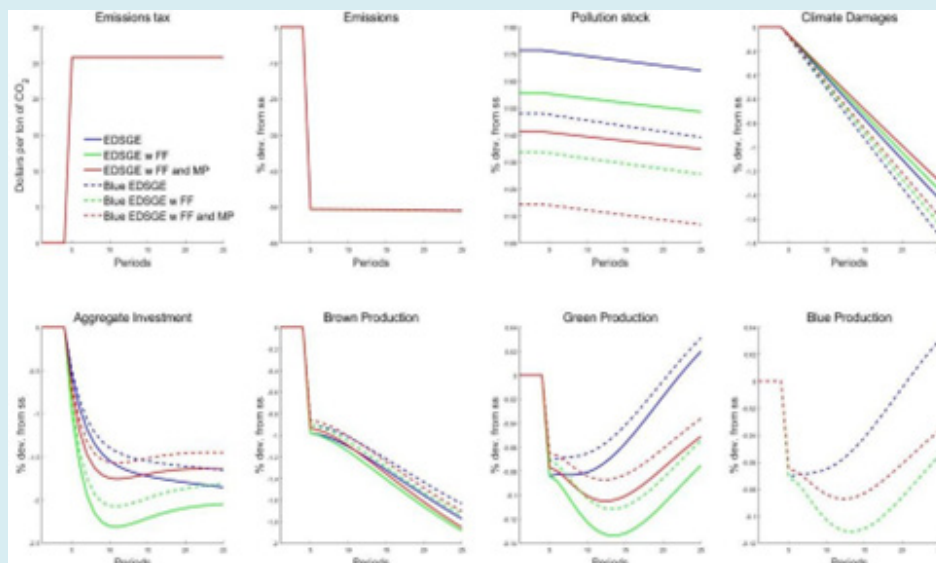
Figure 2: Carbon tax increased to 0.0288.
