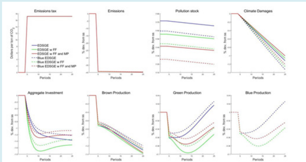
Figure 9: Carbon capture decreased to 0.4.
