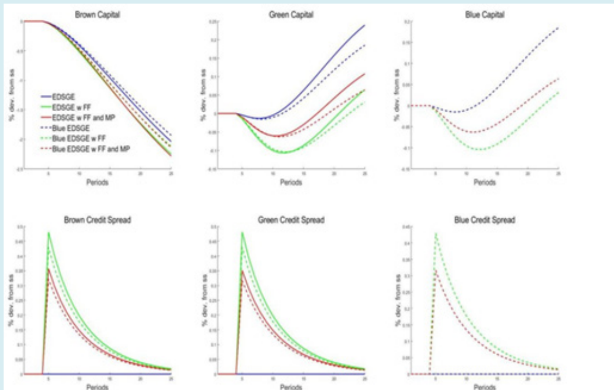
Figure 4: Carbon tax increased to 0.0288.
