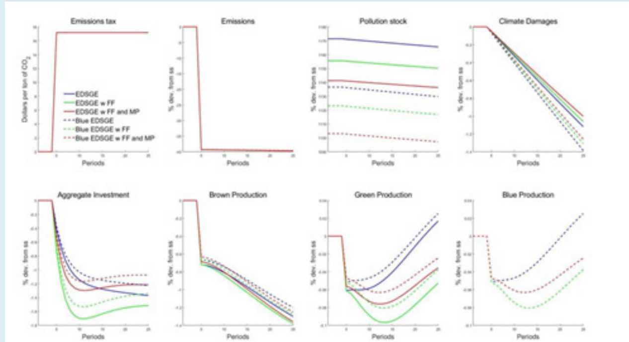
Figure 8: Carbon capture increased to 0.6.
