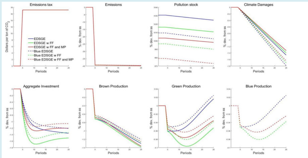
Figure 7: Pollution decay decreased to 0.996.
