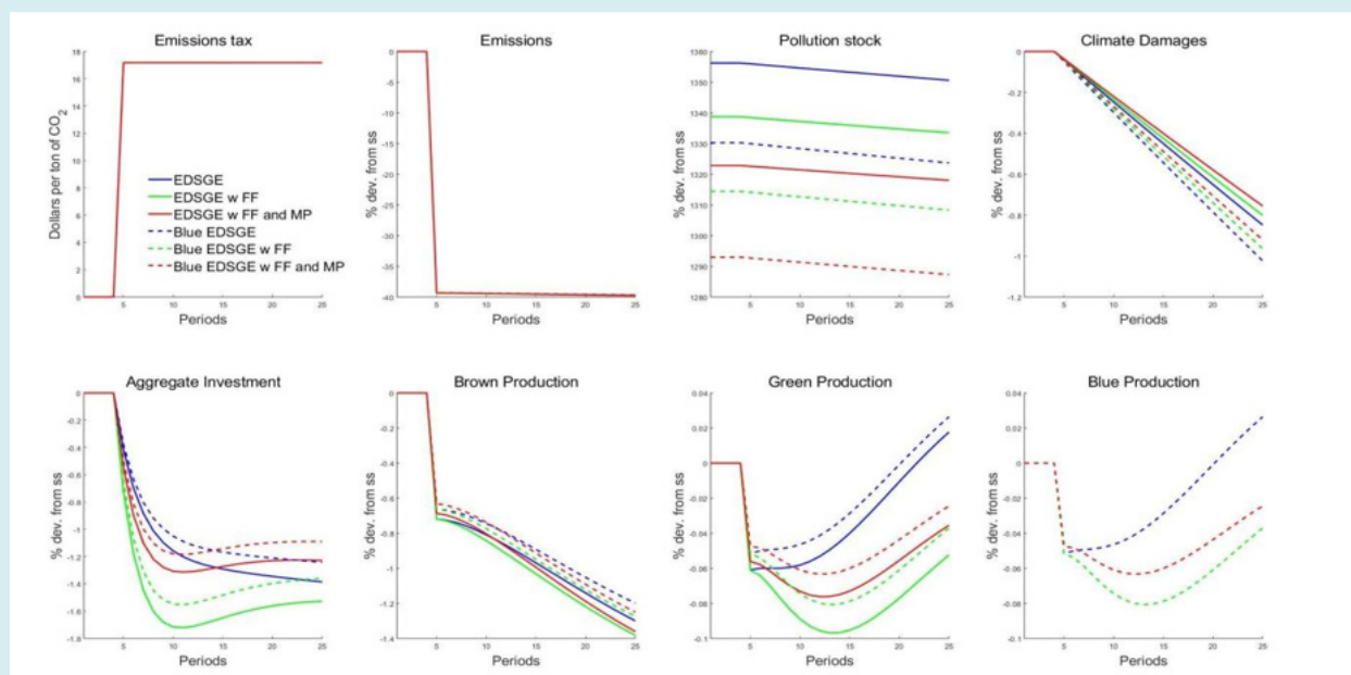
Figure 6: Pollution decay increased to 0.997.
