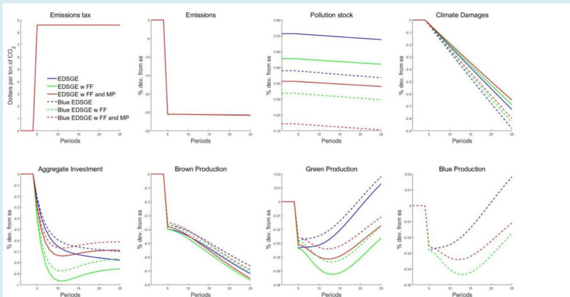
Figure 3: Carbon tax decreased to 0.0096.
