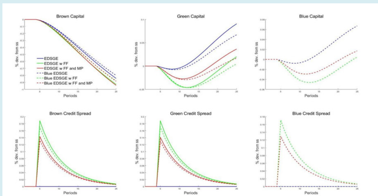
Figure 5: Carbon tax decreased to 0.0096.
